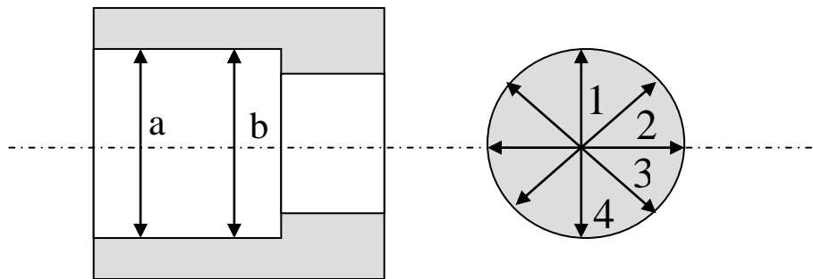
Housing Seats
